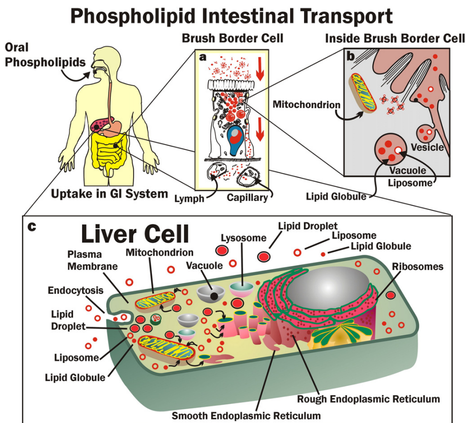
Fig. 1. Some phospholipid transport systems involved in delivery of MLR phospholipids to intracellular membranes. Most orally ingested phospholipids are initially absorbed and transported in the upper small intestines by brush border epithelial cells after their dispersion and enzymatic digestion. (a) MLR phospholipids are usually protected from complete disruption and enzymatic degradation by bound fructooligosaccharides, permitting transportation into cells as small glycerolphospholipid micelles, vesicles, globules and other forms by endocytotic processes. At the distal or basolateral regions of the brush border cells excess lipid vesicles and globules can be extruded by a reverse exocytotic/pinocytotic process and eventually transported to lymph and blood vessels. (b) The endocytotic transport of lipid droplets and vesicles into brush border epithelial cells is shown in more detail. In addition, some of the phospholipids are absorbed by the epithelial cell plasma membrane and transported as simple phospholipids or their degradation products by phospholipid carrier molecules to organelle membranes, including mitochondria. (c) A liver cells is shown with internal lipid micelles, vesicles, globules and lipid droplets. These structures can bind to various intracellular membranes and transfer glycerolphospholipids and pick up damaged lipids. Not shown in the figure are lipid transport/transfer by direct membrane-to-membrane contact and lipid droplet-, globule-, and vesicle-to-membrane contact or temporary fusion with intracellular membranes or by protein lipid carriers. (Modified from Nicolson and Ash [3]).
